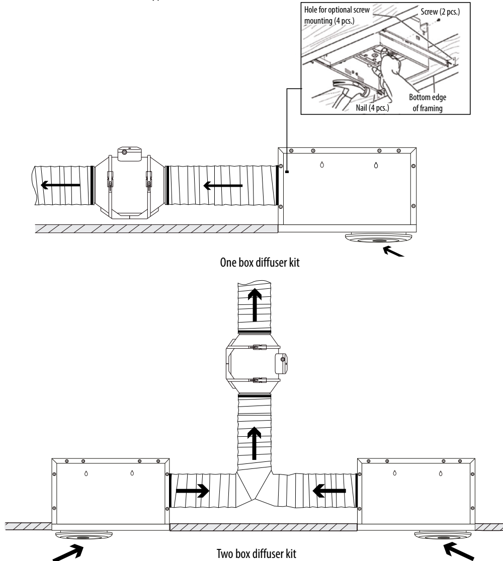
Typical installation of the TT Silnet Kit 100-1L
