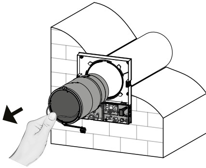
TwinFresh Expert RW1-50
